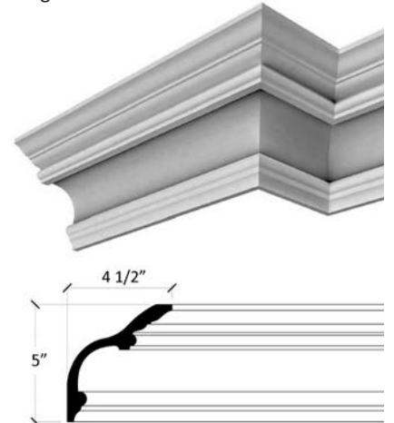
Large Plain Coved Cornice
