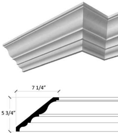
Medium Plain Cornice
