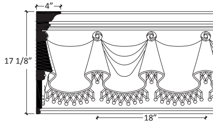
Ornate cornice
